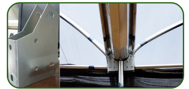
Gutter Jointer
